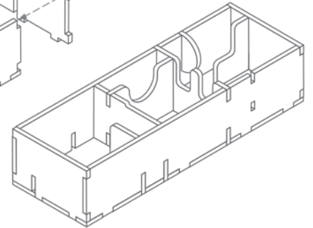
Finished tray
